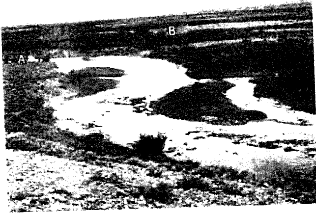
FIGURE 16. A view of a braided section of a tributary of the Ganges, West Bengal, showing a typical braided channel pattern. The white line is a cross-section line drawn across the channel.
