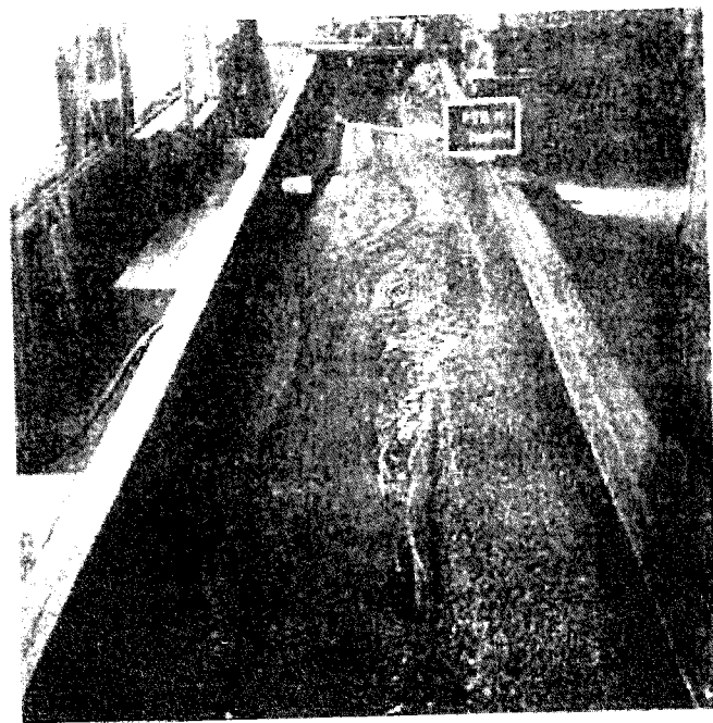
FIGURE 25. Aerial view of the channel at station 14 under 7 hours of flow. The submerged bar is in the 10-pet reach to the left of the section.
