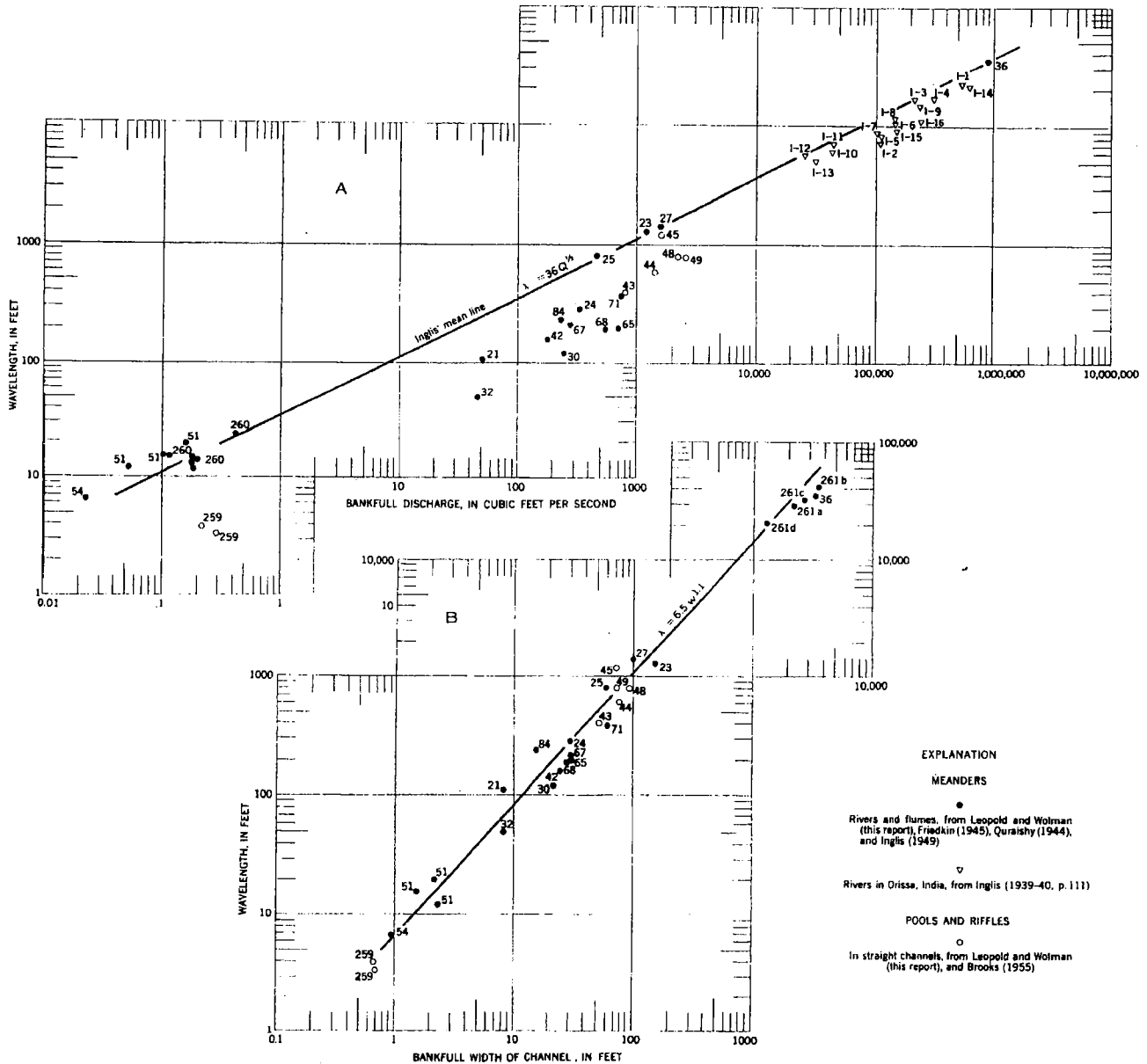
FIGURE 45.—Wavelength of meanders and of riffles as functions of bankfull discharge and channel width.
